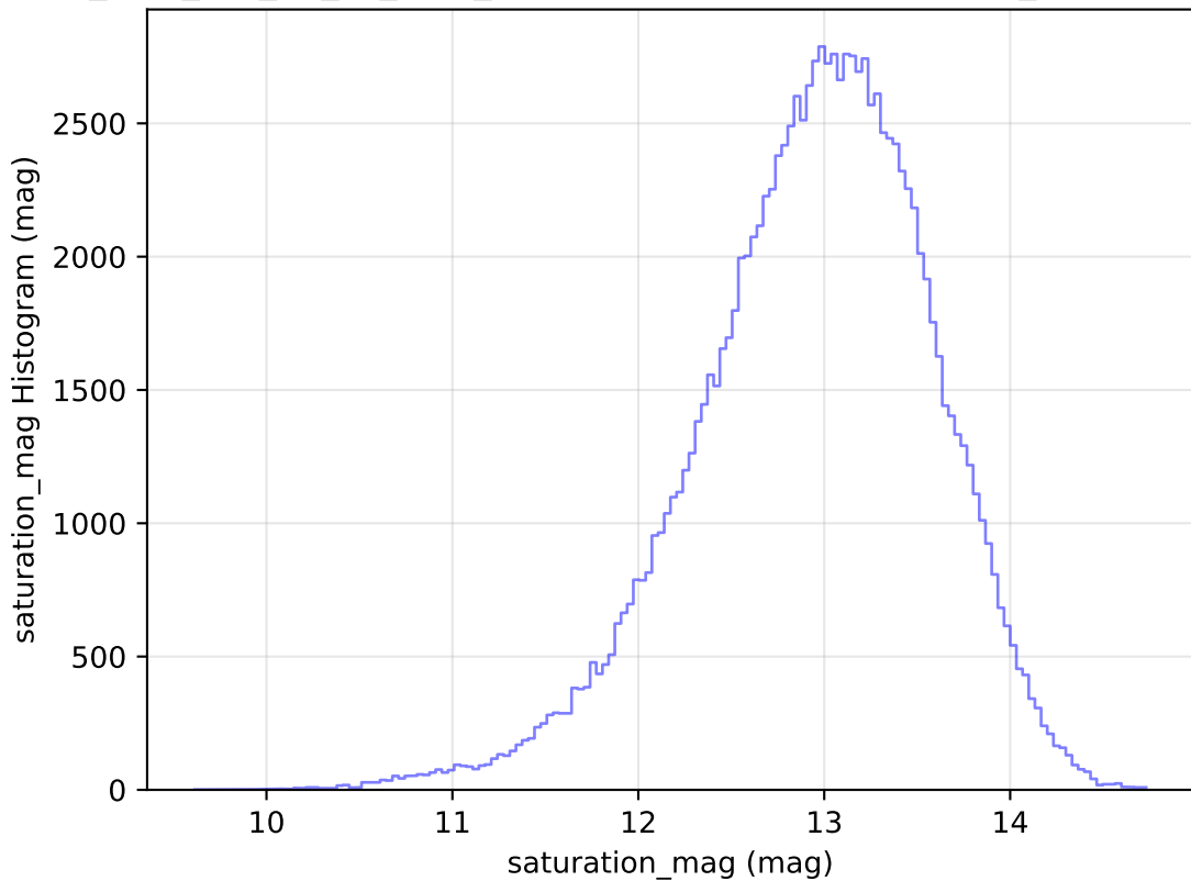
too_elab_r16_d2_gz_v3.4_10yrs WFD u band: saturation_mag Histogram
