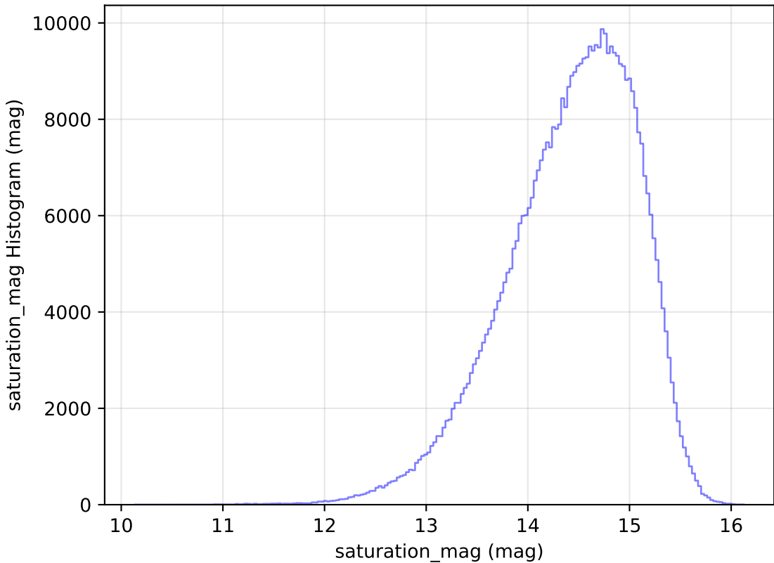
too_elab_r16_d2_gz_v3.4_10yrs WFD i band: saturation_mag Histogram
