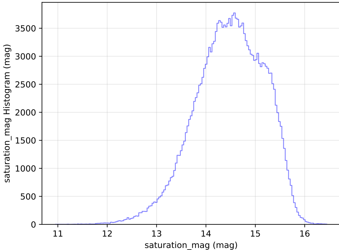
too_elab_r16_d2_gz_v3.4_10yrs WFD g band: saturation_mag Histogram
