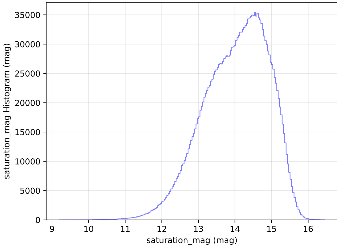
too_elab_r16_d2_gz_v3.4_10yrs WFD all bands: saturation_mag Histogram
