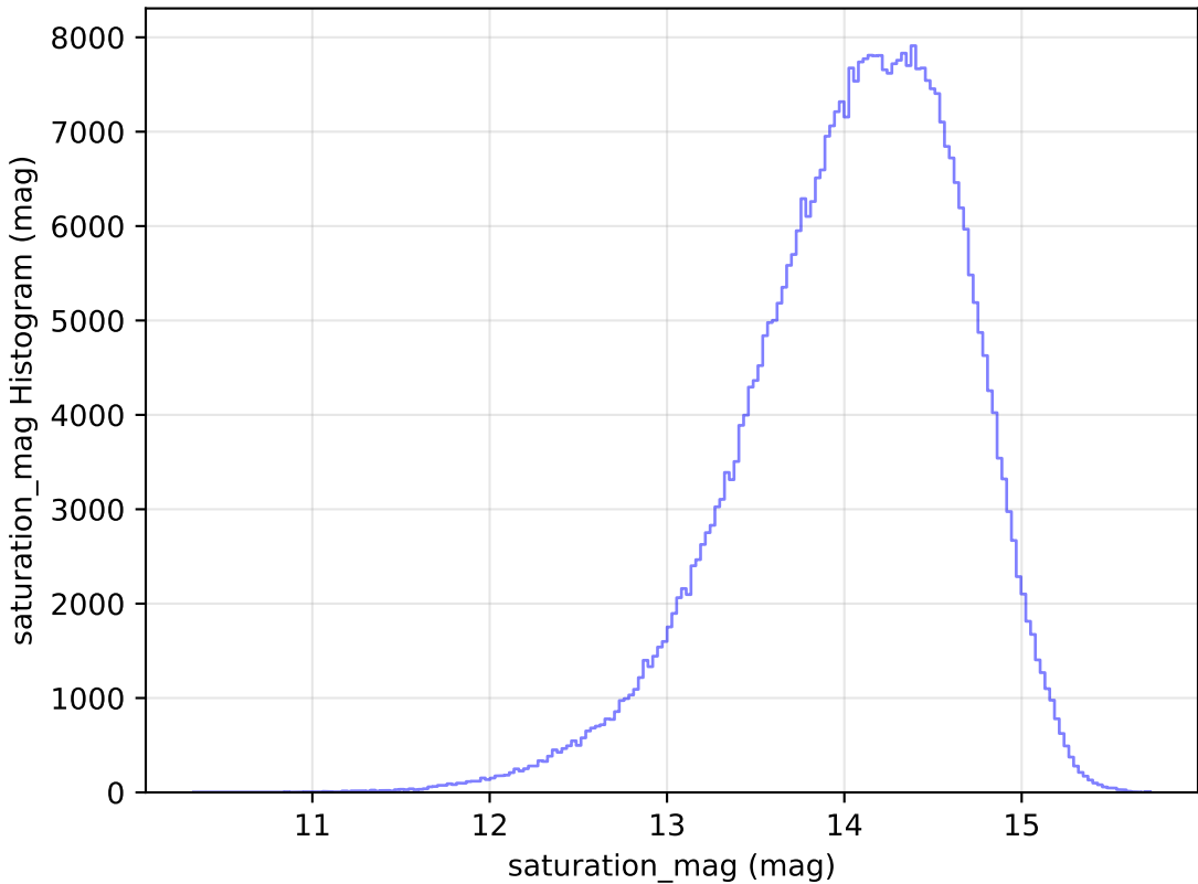
too_elab_r16_d2_gz_v3.4_10yrs All sky z band: saturation_mag Histogram
