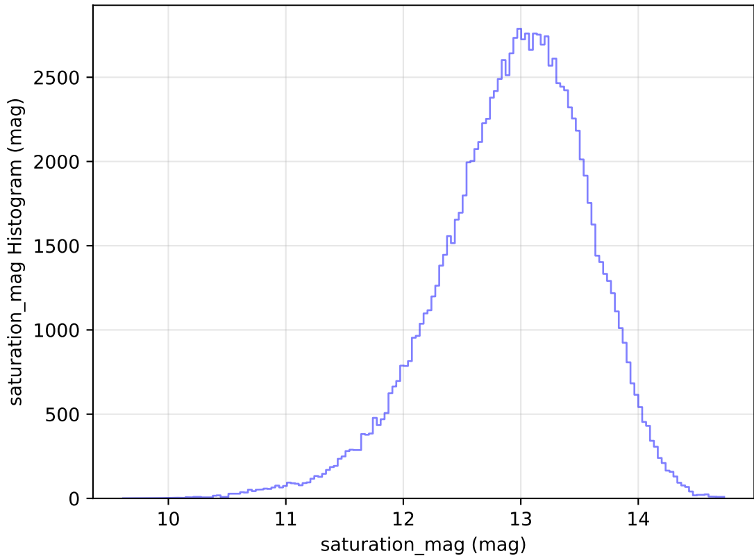
too_elab_r16_d2_gz_v3.4_10yrs All sky u band: saturation_mag Histogram
