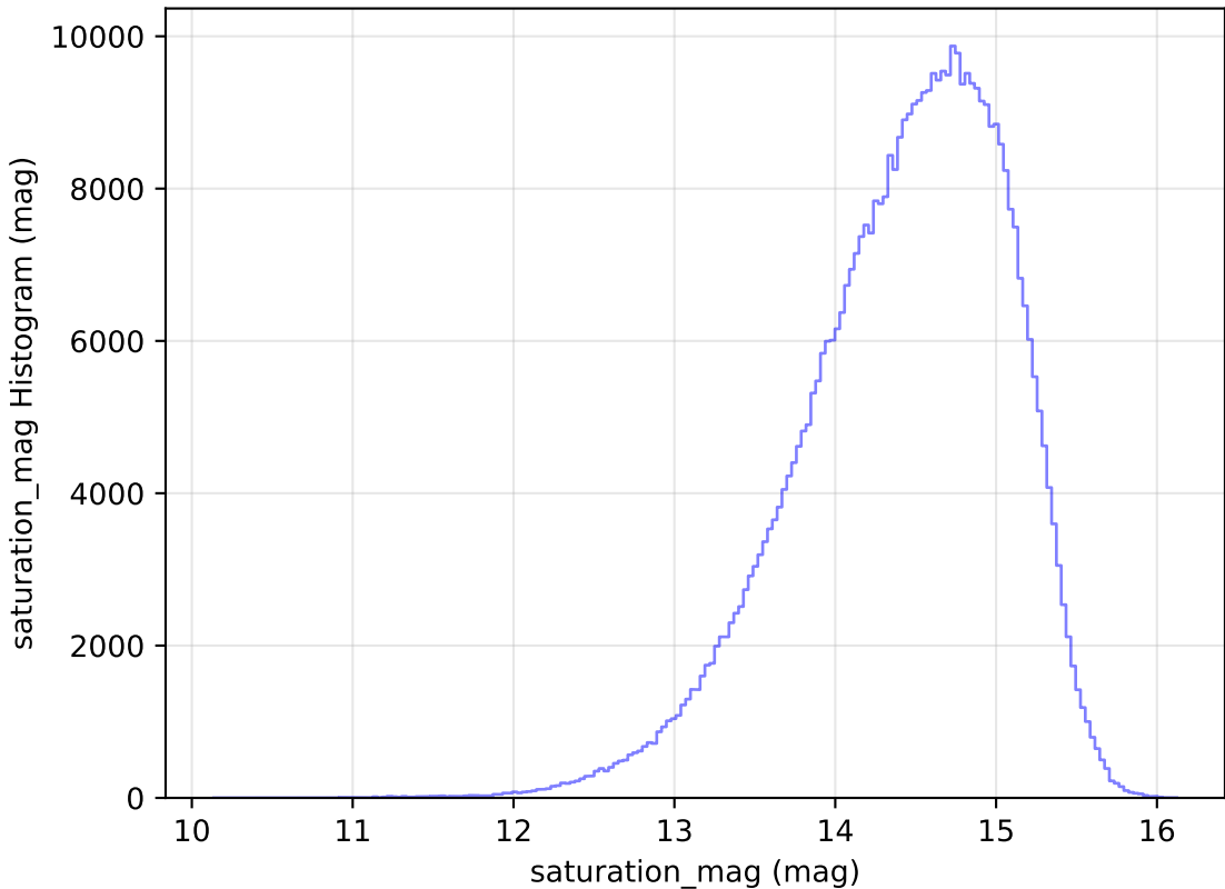
too_elab_r16_d2_gz_v3.4_10yrs All sky i band: saturation_mag Histogram
