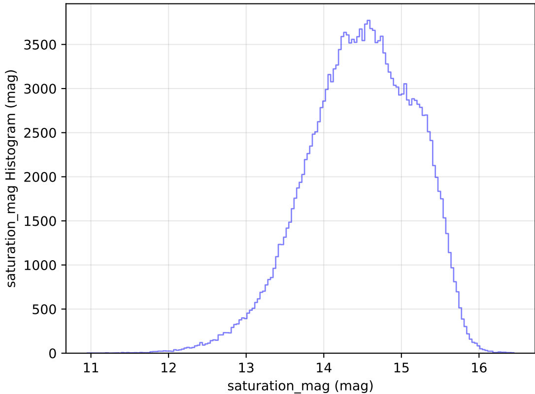
too_elab_r16_d2_gz_v3.4_10yrs All sky g band: saturation_mag Histogram
