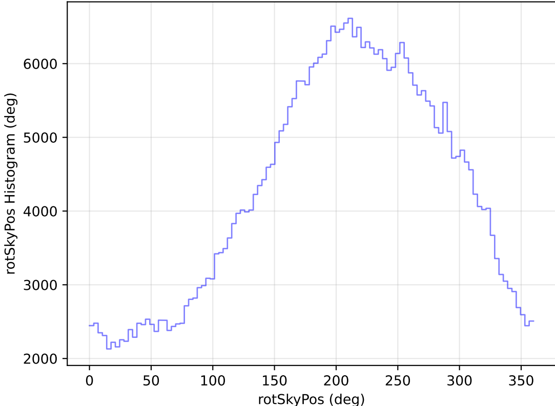
too_elab_r16_d2_gz_v3.4_10yrs WFD z band: rotSkyPos Histogram
