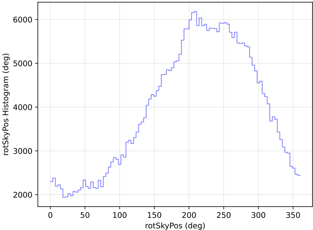
too_elab_r16_d2_gz_v3.4_10yrs WFD y band: rotSkyPos Histogram
