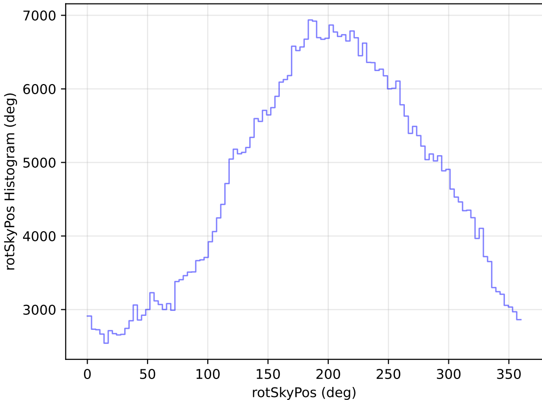
too_elab_r16_d2_gz_v3.4_10yrs WFD r band: rotSkyPos Histogram
