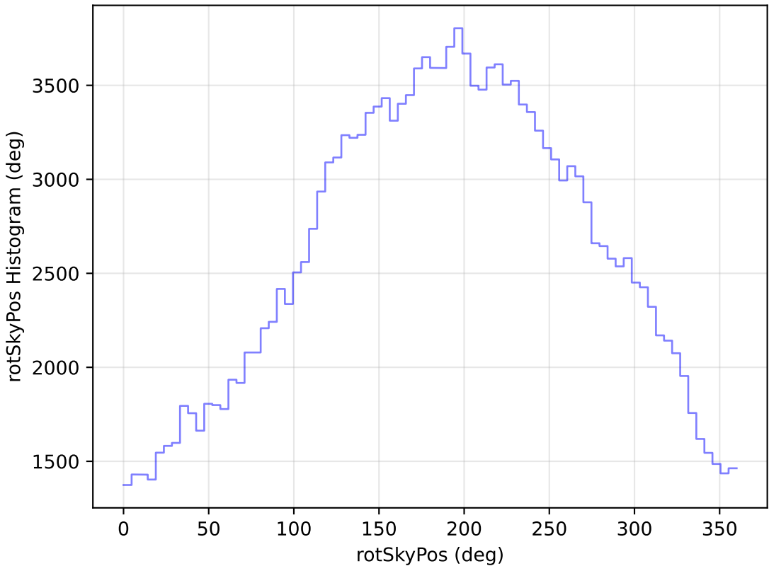
too_elab_r16_d2_gz_v3.4_10yrs WFD g band: rotSkyPos Histogram
