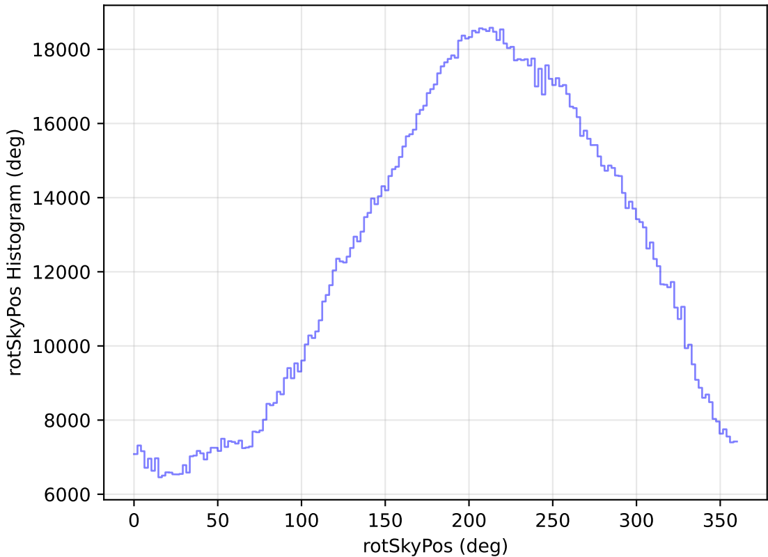
too_elab_r16_d2_gz_v3.4_10yrs WFD all bands: rotSkyPos Histogram
