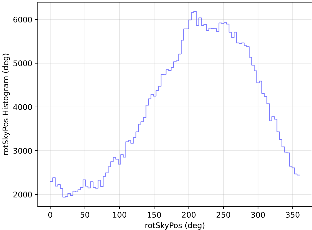
too_elab_r16_d2_gz_v3.4_10yrs All sky y band: rotSkyPos Histogram
