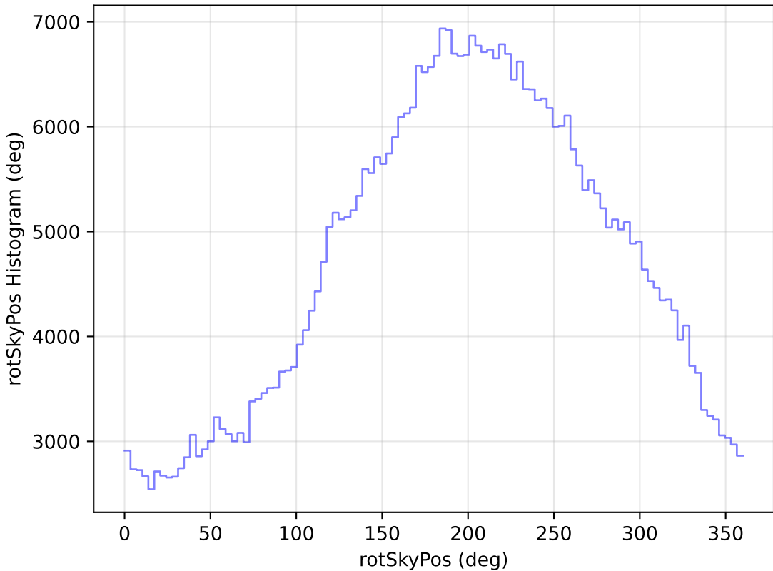
too_elab_r16_d2_gz_v3.4_10yrs All sky r band: rotSkyPos Histogram
