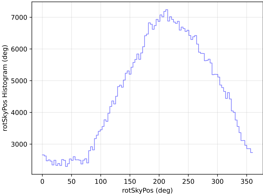
too_elab_r16_d2_gz_v3.4_10yrs All sky i band: rotSkyPos Histogram
