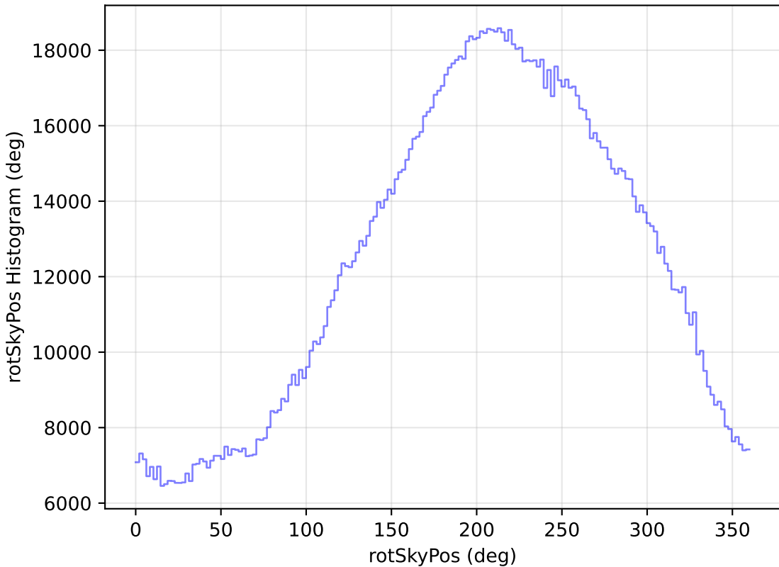
too_elab_r16_d2_gz_v3.4_10yrs All sky all bands: rotSkyPos Histogram
