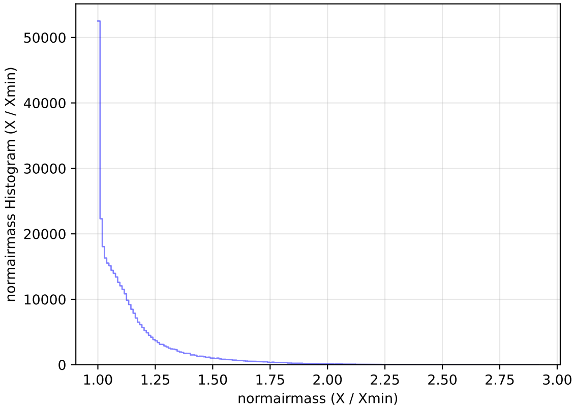
too_elab_r16_d2_gz_v3.4_10yrs WFD y band: normairmass Histogram
