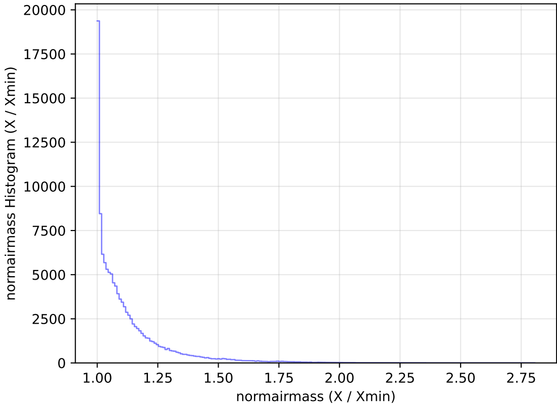
too_elab_r16_d2_gz_v3.4_10yrs WFD u band: normairmass Histogram
