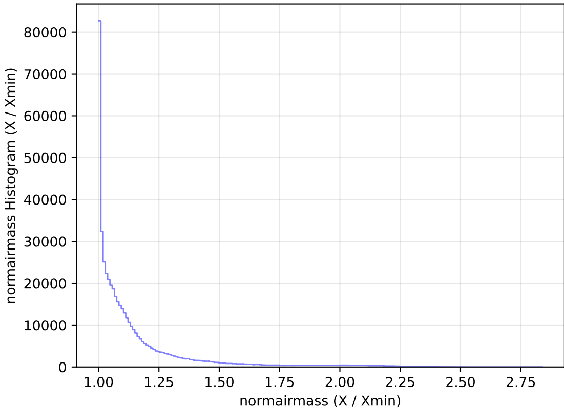
too_elab_r16_d2_gz_v3.4_10yrs WFD r band: normairmass Histogram
