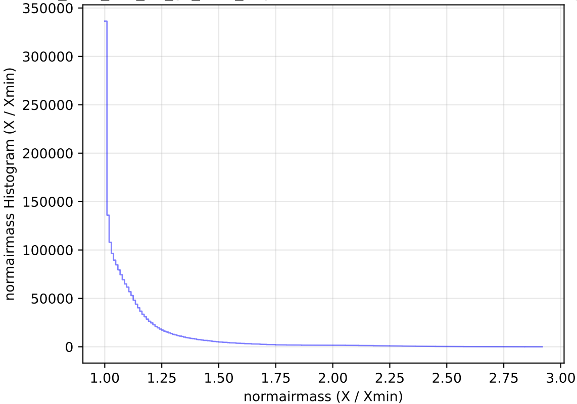
too_elab_r16_d2_gz_v3.4_10yrs WFD all bands: normairmass Histogram
