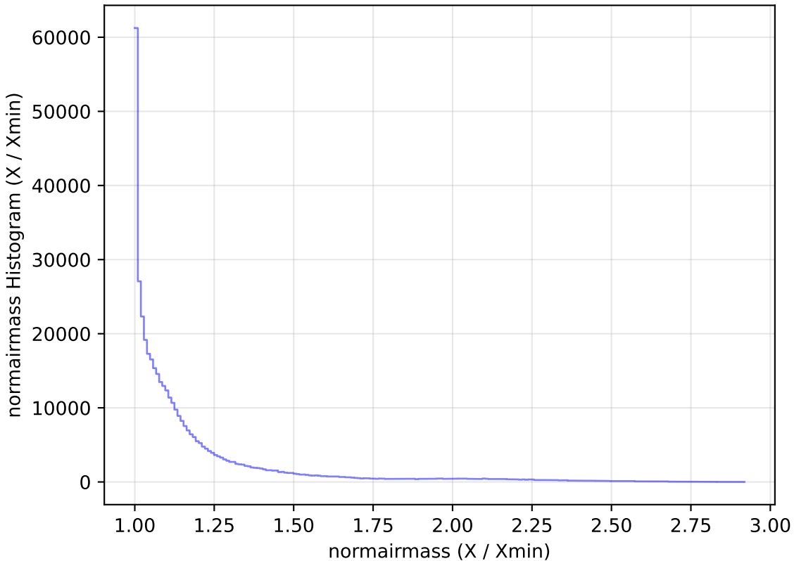
too_elab_r16_d2_gz_v3.4_10yrs All sky z band: normairmass Histogram
