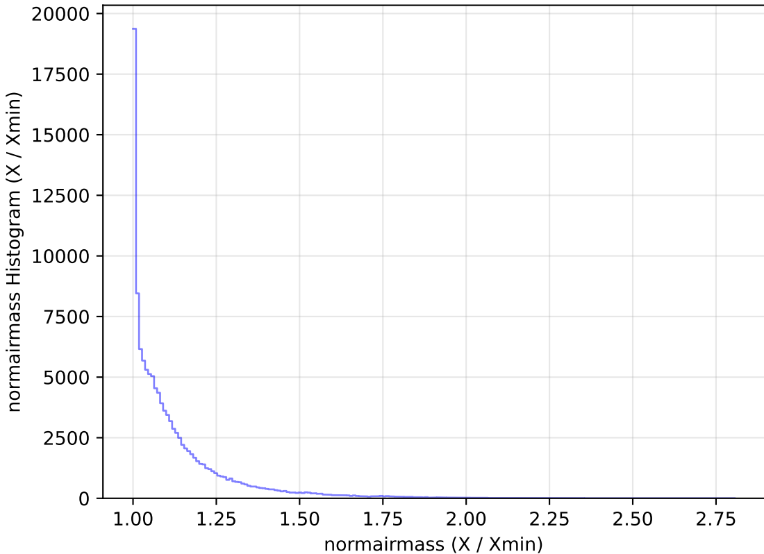
too_elab_r16_d2_gz_v3.4_10yrs All sky u band: normairmass Histogram
