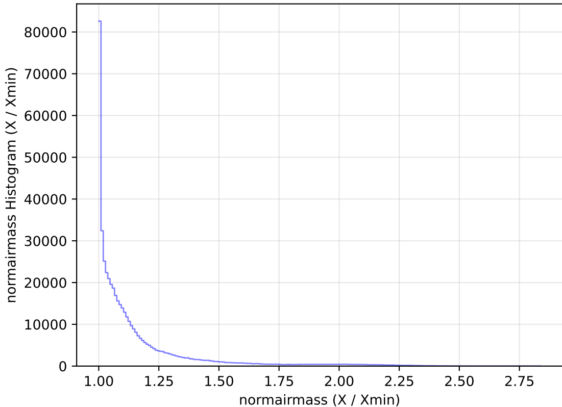
too_elab_r16_d2_gz_v3.4_10yrs All_sky r band: normairmass Histogram
