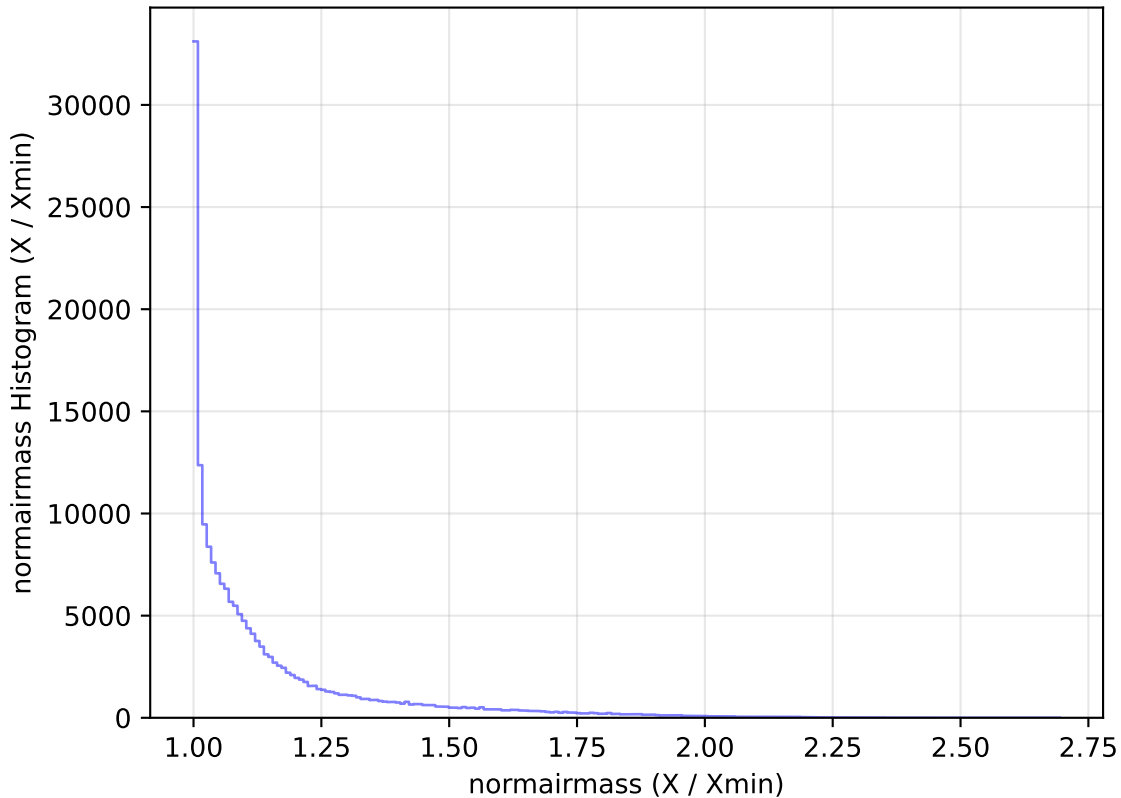
too_elab_r16_d2_gz_v3.4_10yrs All sky g band: normairmass Histogram
