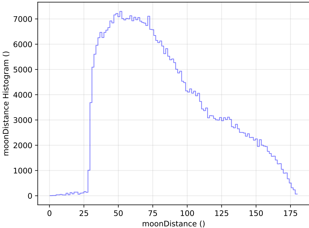
too_elab_r16_d2_gz_v3.4_10yrs WFD z band: moonDistance Histogram
