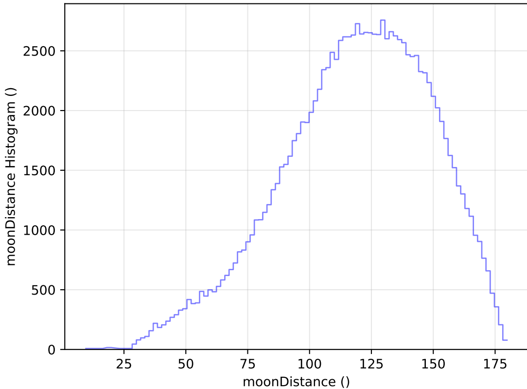
too_elab_r16_d2_gz_v3.4_10yrs WFD u band: moonDistance Histogram
