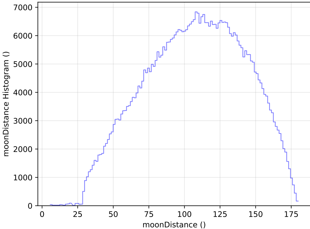
too_elab_r16_d2_gz_v3.4_10yrs WFD r band: moonDistance Histogram
