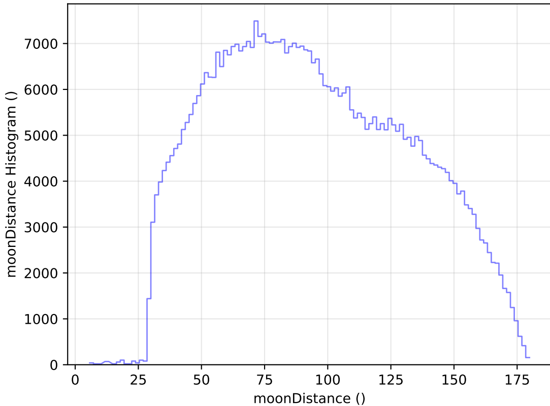
too_elab_r16_d2_gz_v3.4_10yrs WFD i band: moonDistance Histogram
