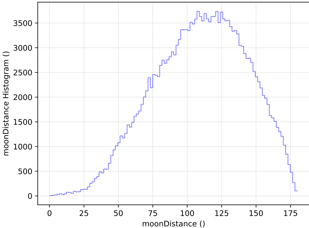
too_elab_r16_d2_gz_v3.4_10yrs WFD g band: moonDistance Histogram
