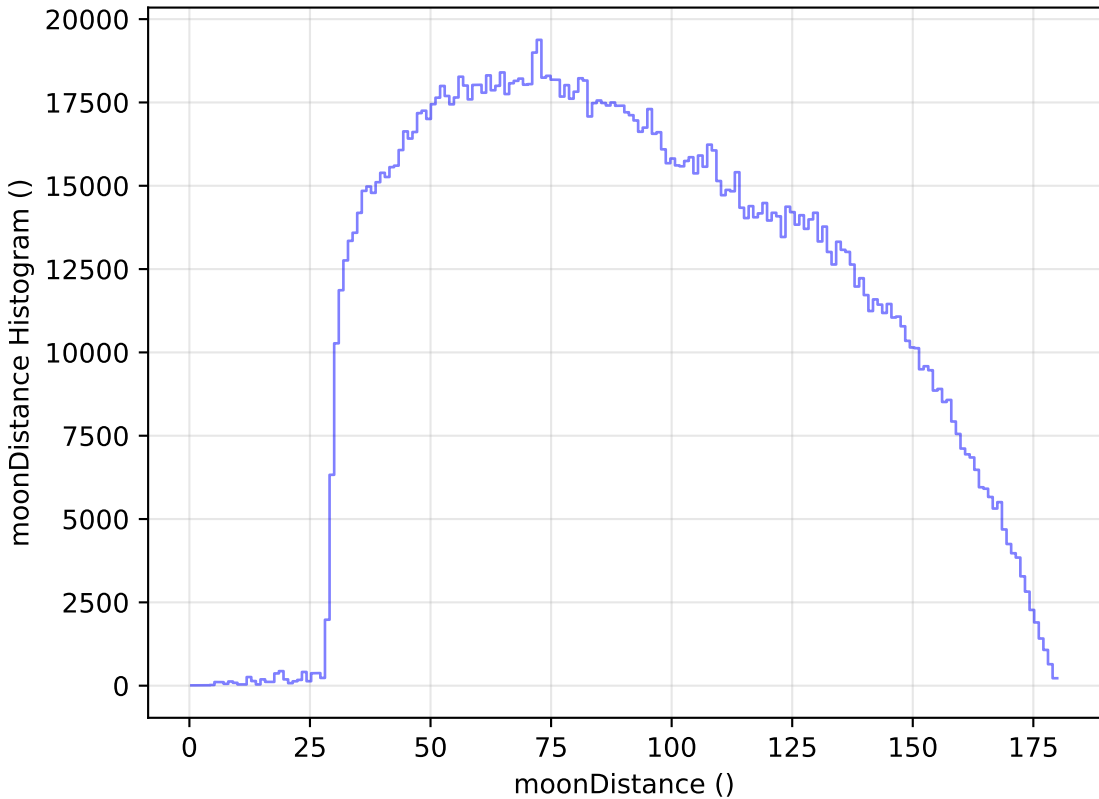
too_elab_r16_d2_gz_v3.4_10yrs WFD all bands: moonDistance Histogram
