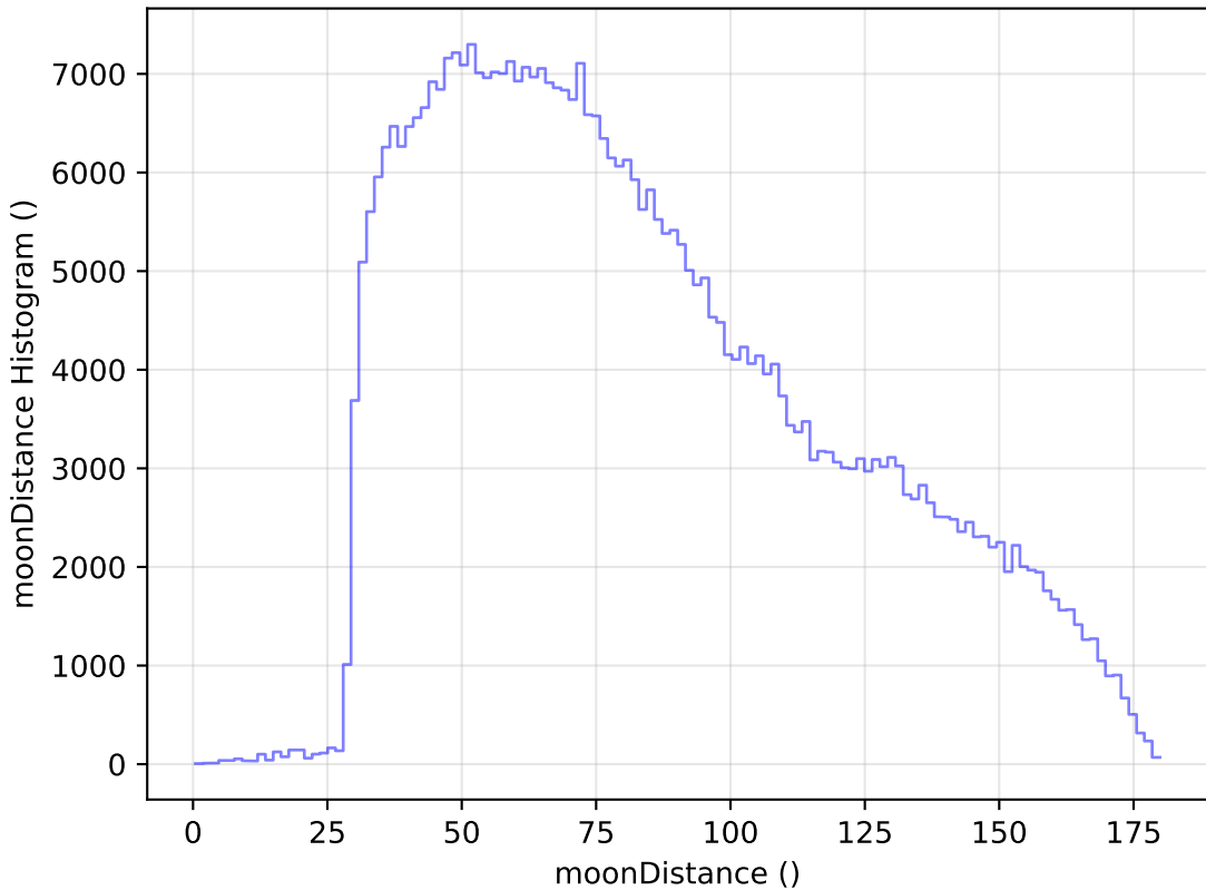
too_elab_r16_d2_gz_v3.4_10yrs All sky z band: moonDistance Histogram
