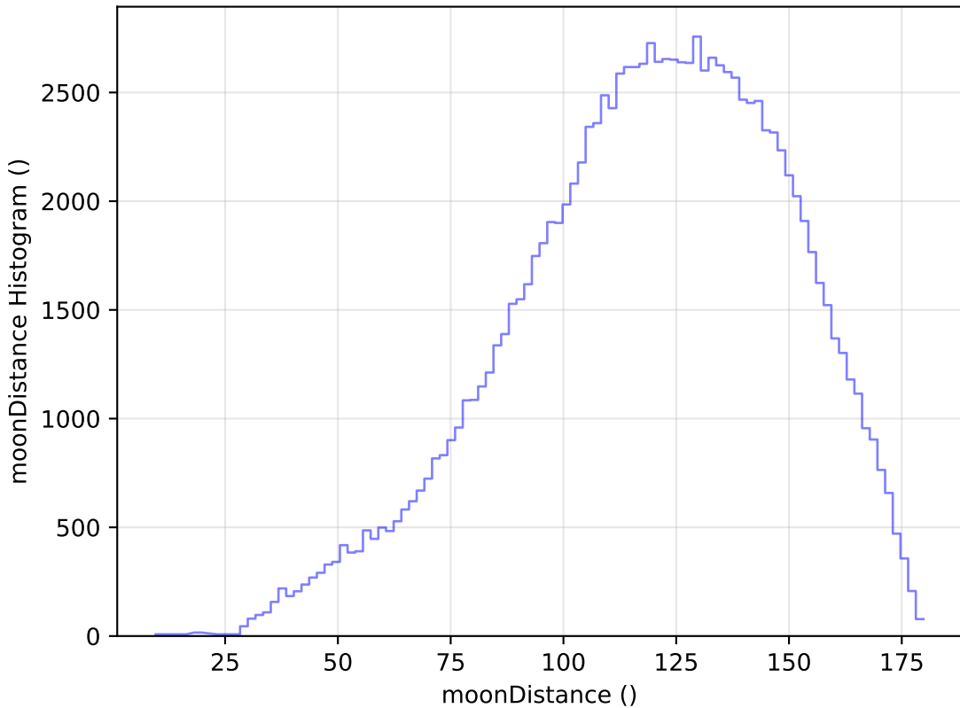
too_elab_r16_d2_gz_v3.4_10yrs All sky u band: moonDistance Histogram
