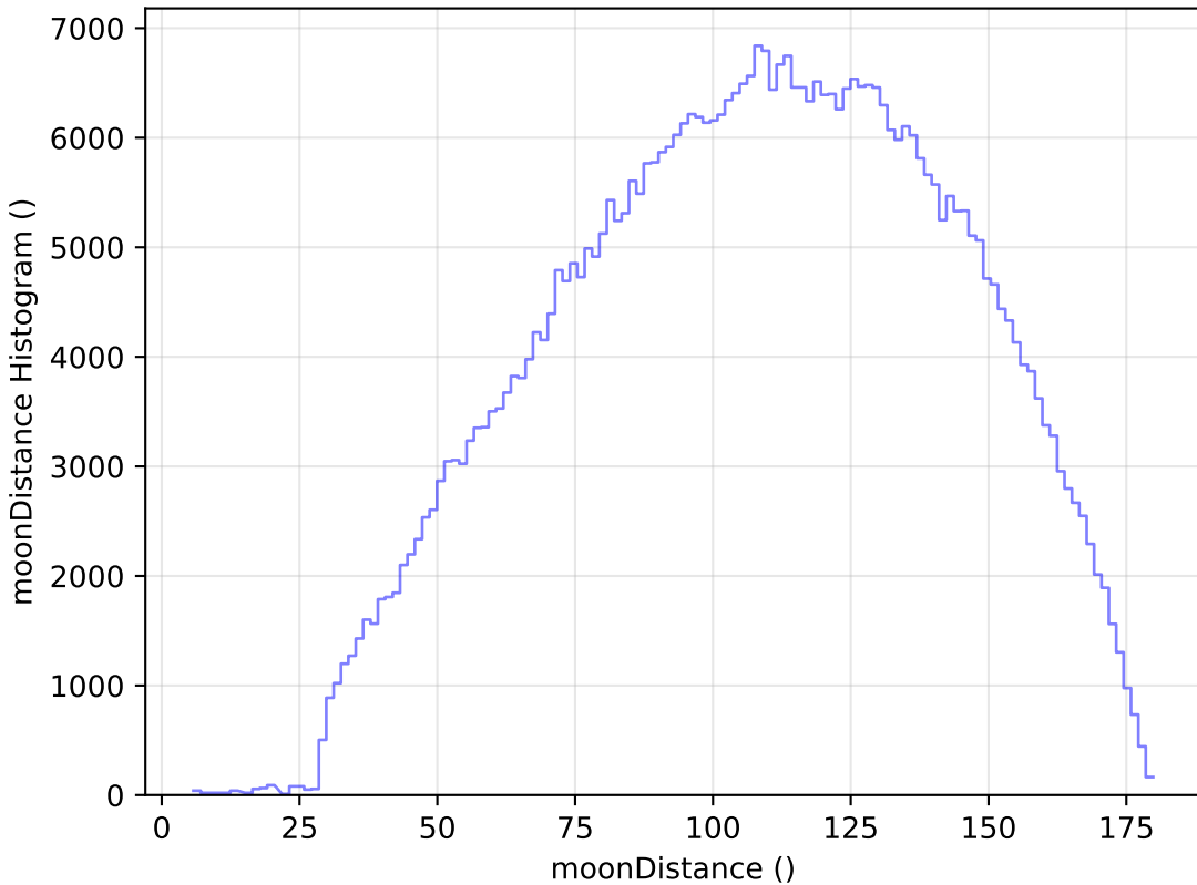
too_elab_r16_d2_gz_v3.4_10yrs All sky r band: moonDistance Histogram
