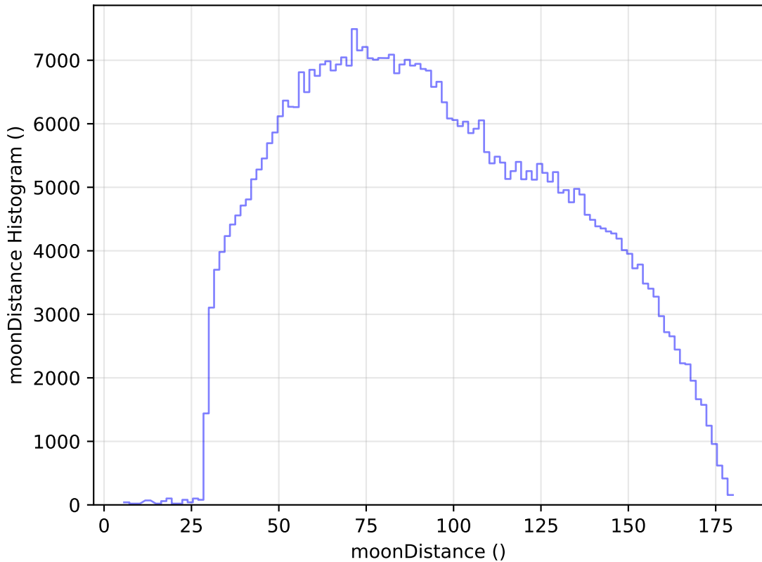
too_elab_r16_d2_gz_v3.4_10yrs All sky i band: moonDistance Histogram
