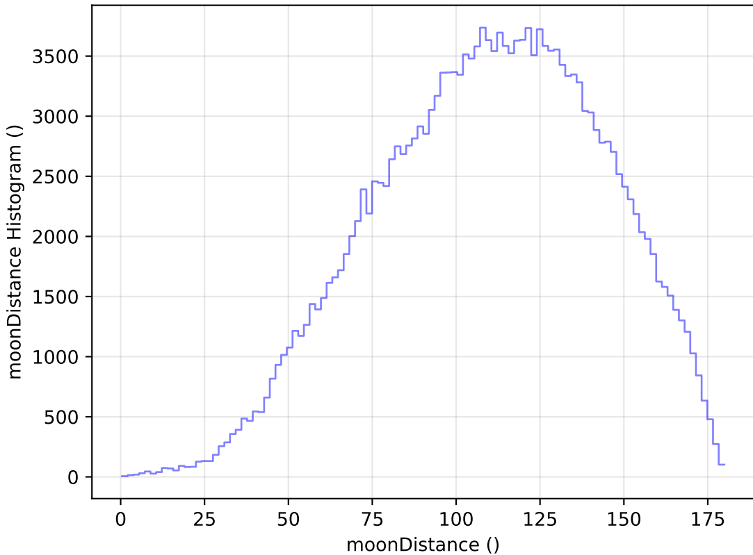
too_elab_r16_d2_gz_v3.4_10yrs All sky g band: moonDistance Histogram
