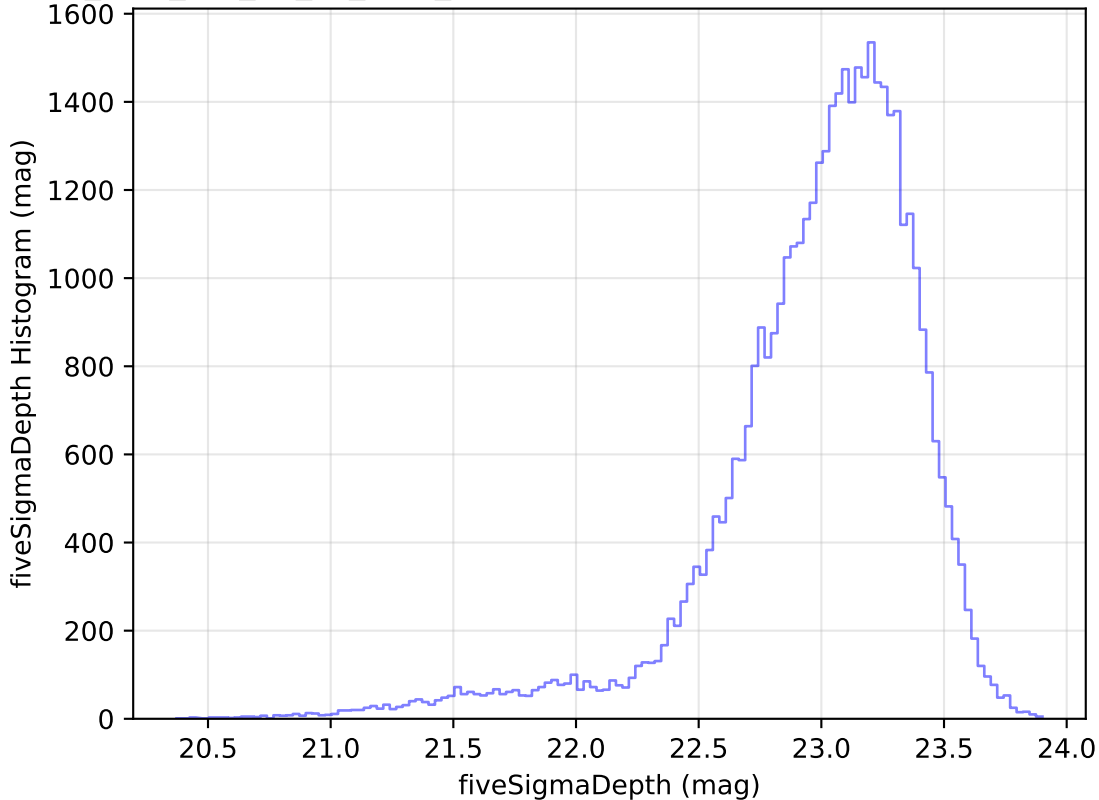
too_elab_r16_d2_gz_v3.4_10yrs Yr 1 z band: fiveSigmaDepth Histogram
