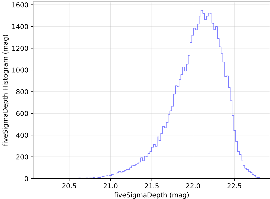
too_elab_r16_d2_gz_v3.4_10yrs Yr 1 y band: fiveSigmaDepth Histogram
