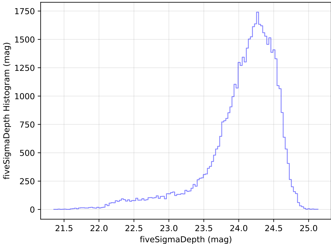
too_elab_r16_d2_gz_v3.4_10yrs Yr 1 r band: fiveSigmaDepth Histogram
