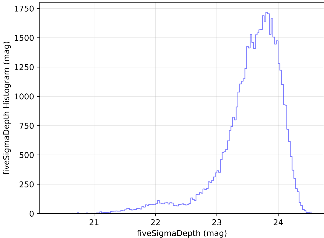
too_elab_r16_d2_gz_v3.4_10yrs Yr 1 i band: fiveSigmaDepth Histogram
