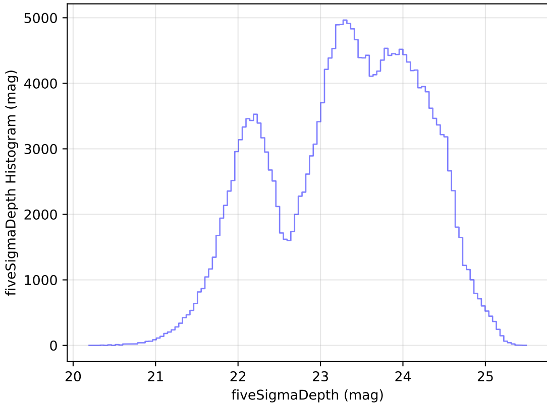
too_elab_r16_d2_gz_v3.4_10yrs Yr 1 all bands: fiveSigmaDepth Histogram
