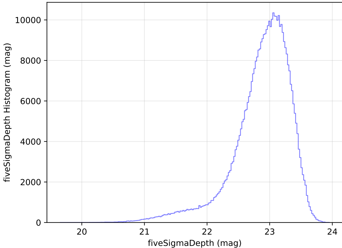
too_elab_r16_d2_gz_v3.4_10yrs WFD z band: fiveSigmaDepth Histogram
