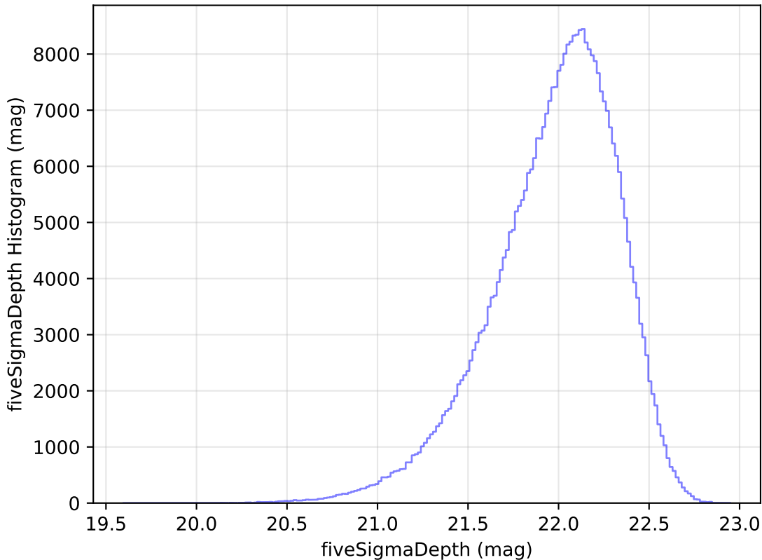
too_elab_r16_d2_gz_v3.4_10yrs WFD y band: fiveSigmaDepth Histogram
