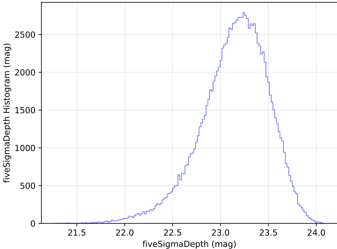
too_elab_r16_d2_gz_v3.4_10yrs WFD u band: fiveSigmaDepth Histogram
