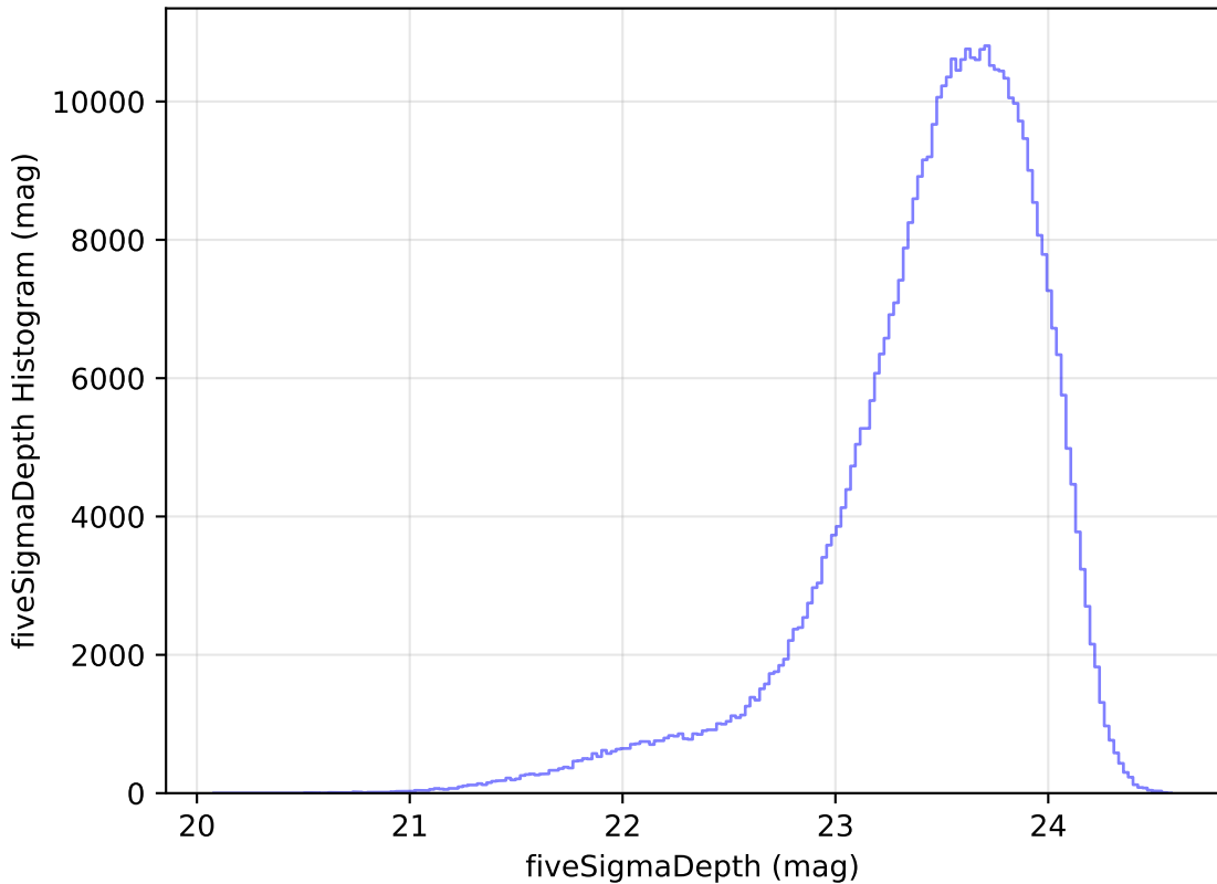
too_elab_r16_d2_gz_v3.4_10yrs WFD i band: fiveSigmaDepth Histogram
