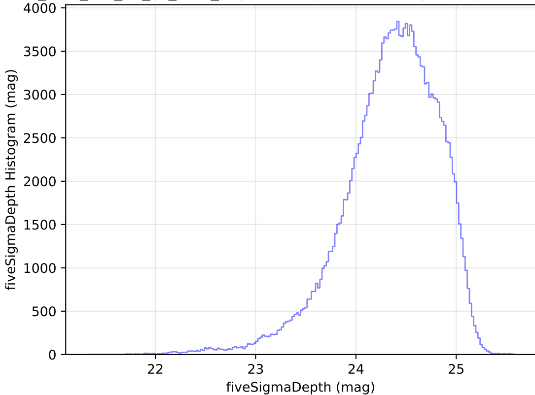
too_elab_r16_d2_gz_v3.4_10yrs WFD g band: fiveSigmaDepth Histogram
