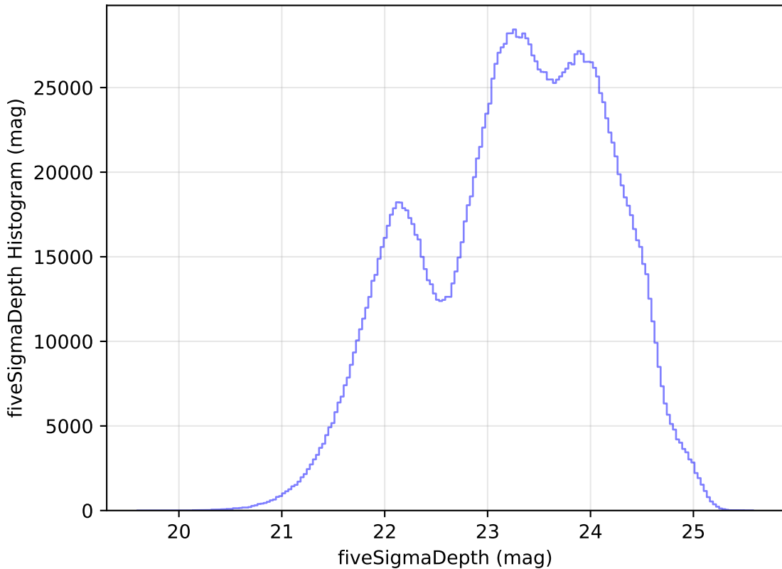
too_elab_r16_d2_gz_v3.4_10yrs WFD all bands: fiveSigmaDepth Histogram
