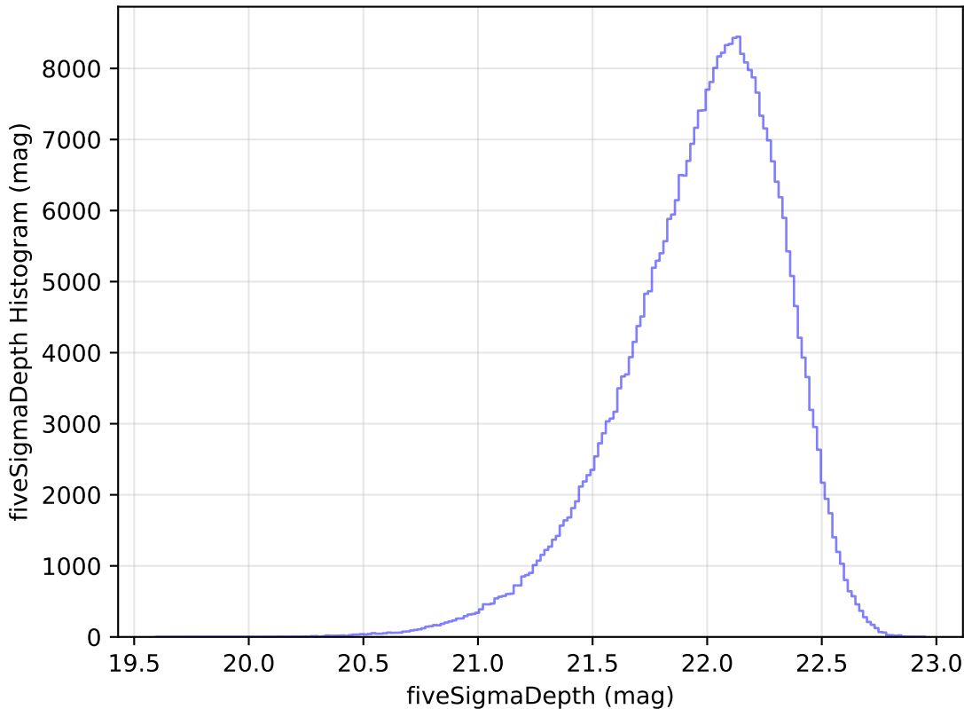
too_elab_r16_d2_gz_v3.4_10yrs All sky y band: fiveSigmaDepth Histogram
