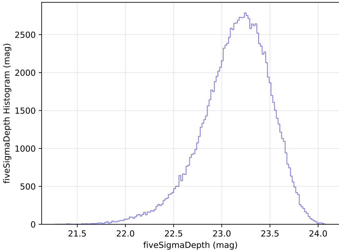
too_elab_r16_d2_gz_v3.4_10yrs All sky u band: fiveSigmaDepth Histogram
