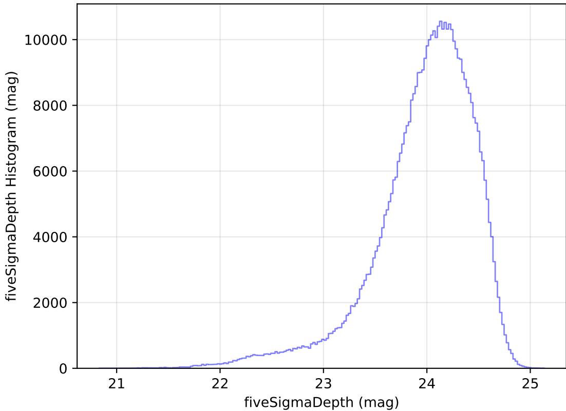
too_elab_r16_d2_gz_v3.4_10yrs All sky r band: fiveSigmaDepth Histogram
